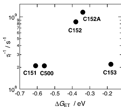
Figure 6. Inverse fluorescence lifetimes of the coumarins in DMSO/GLY at 10 cP as a function of the driving force for ET with DMA.
